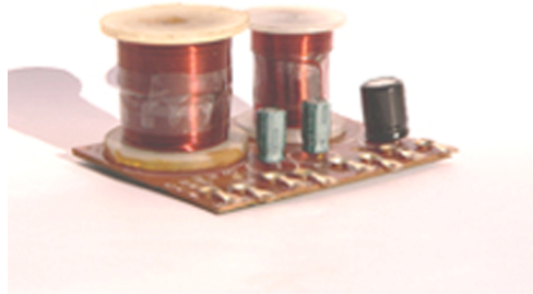
(Crossover Network shown above: 3 way, 6 dB, 40W)
